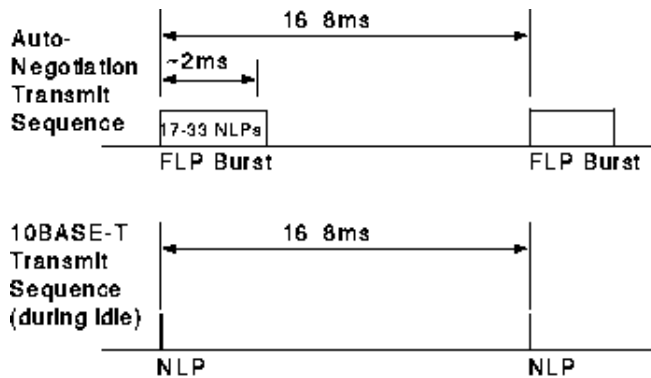
Figure 2. FLP Burst Timing
