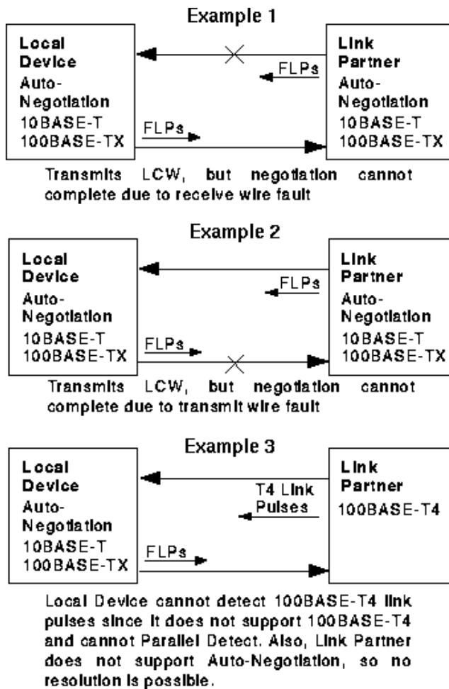
Figure 6. Remote Fault Scenarios
