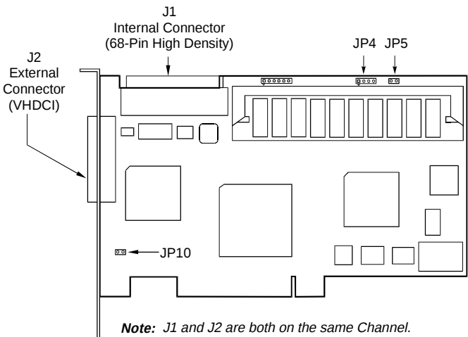
Figure 3-1. AcceleRAID Jumpers and Connectors
