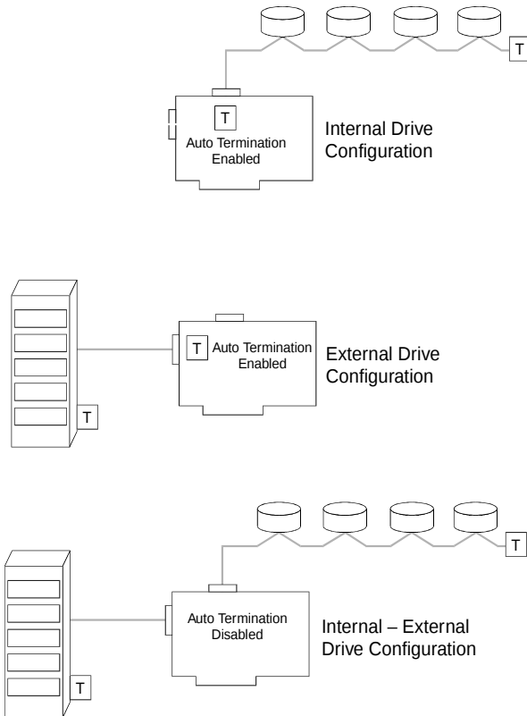
Figure 2-3. AcceleRAID 250 SCSI Termination Examples
