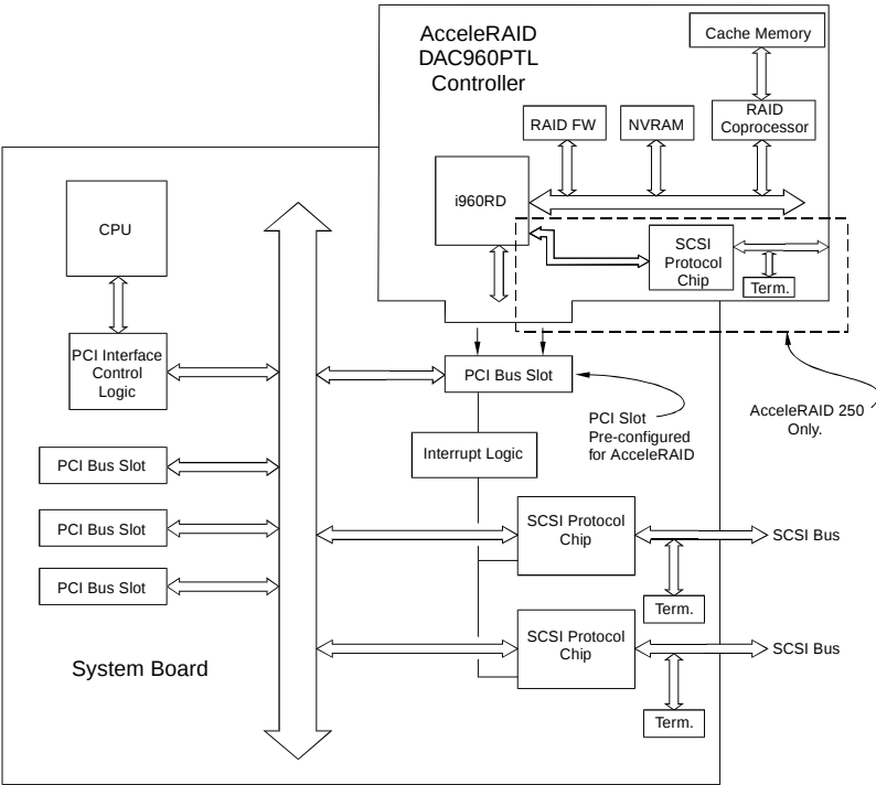
Figure A-1. AcceleRAID and SCSI-Capable System Board
