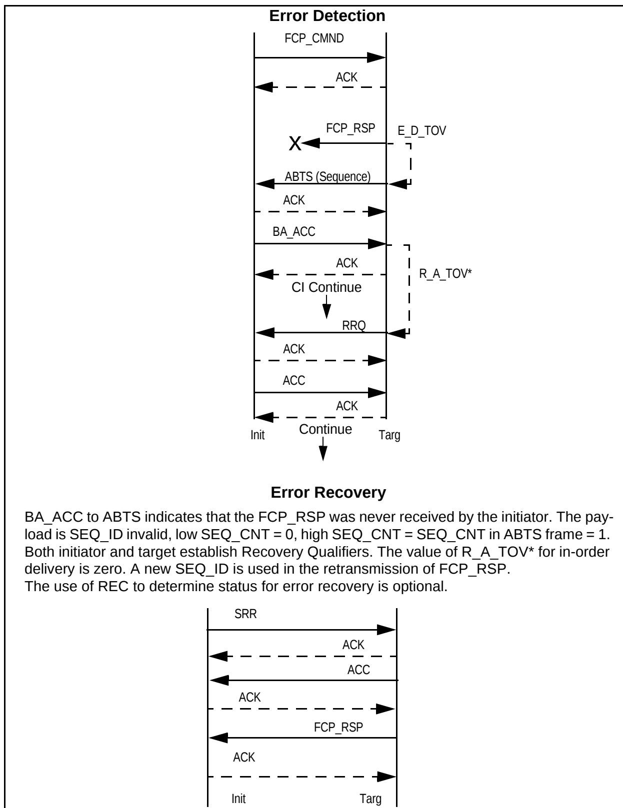
Figure C.9 - FCP_RSP Lost, FCP_CONF not requested, Acknowledged Classes
