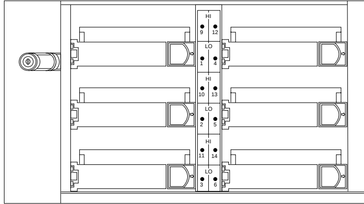
FIGURE B-1 SCSI Address Label on Partition
