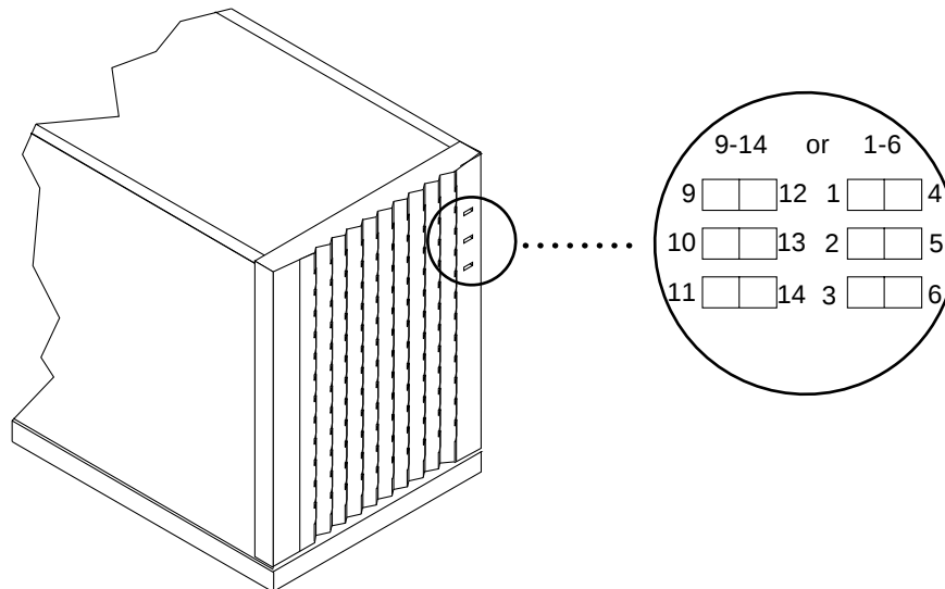
FIGURE 2-1 Front Panel Drive LEDs and SCSI Target Addresses
