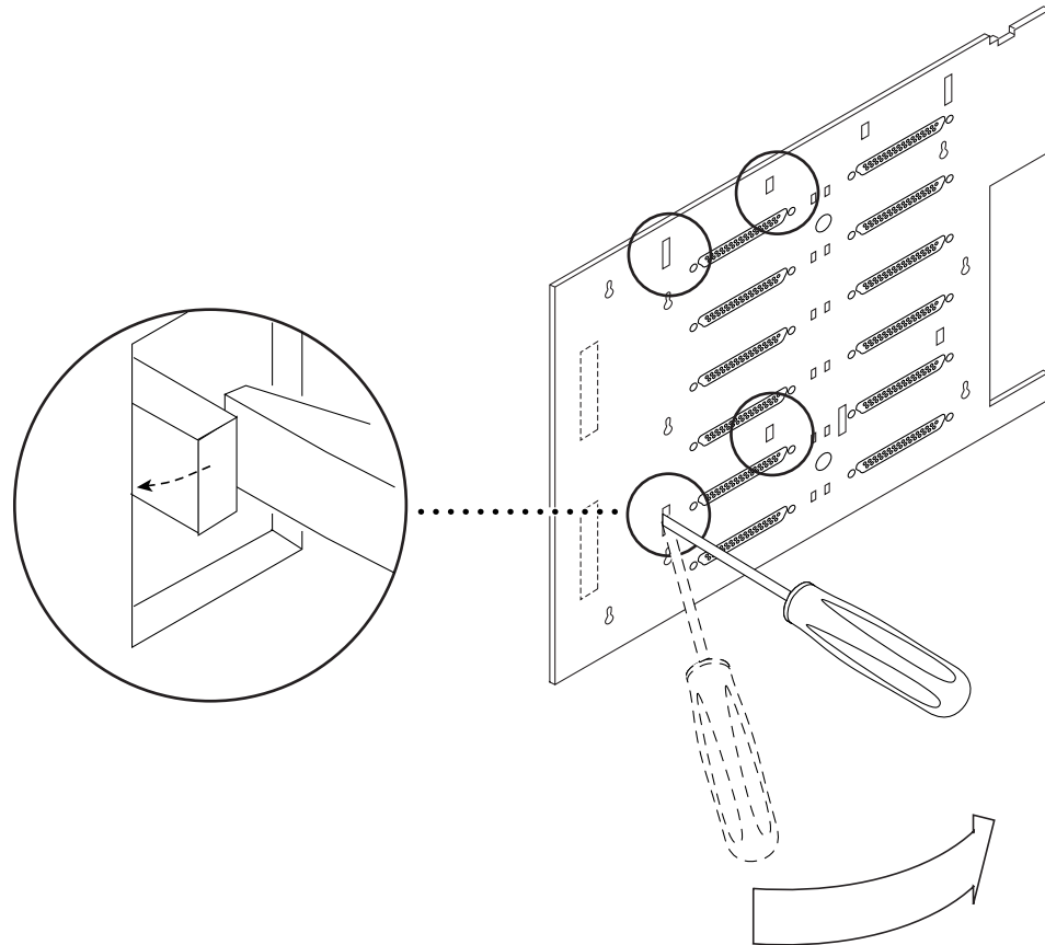
FIGURE 5-6 Unlatching the Tabs on the Left Side
