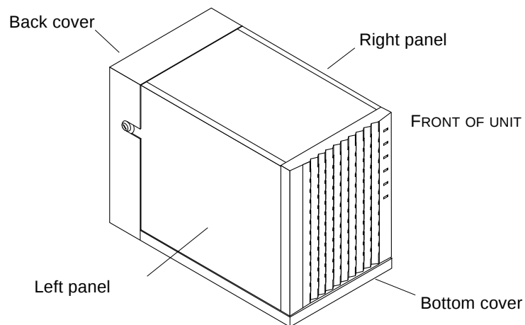
FIGURE 5-1 Removable Covers
