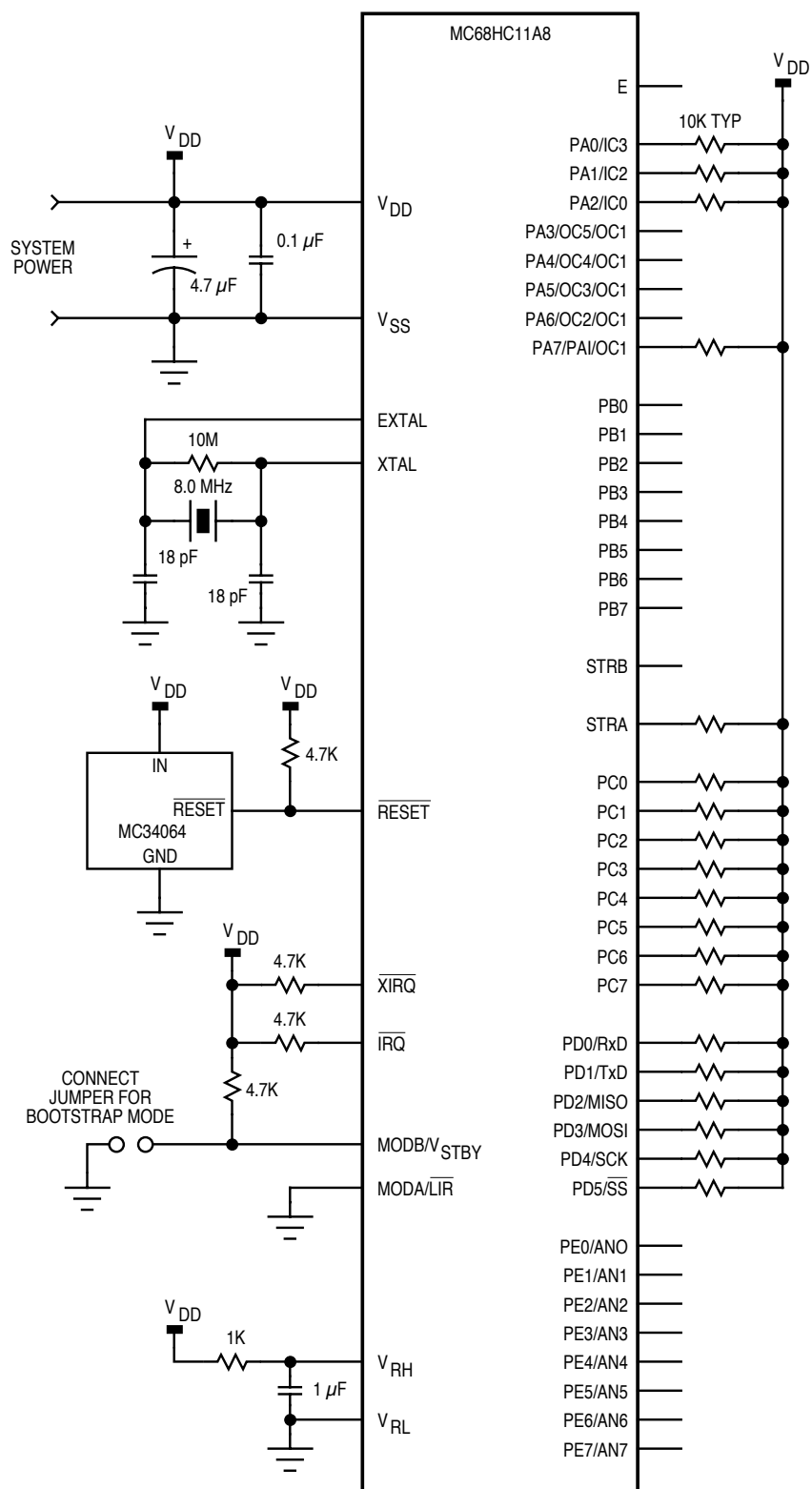
Figure 2-22. Basic Single-Chip Mode Connections
