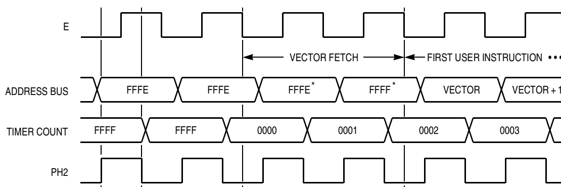
Figure 10-32. Timer Counter as MCU Leaves Reset
