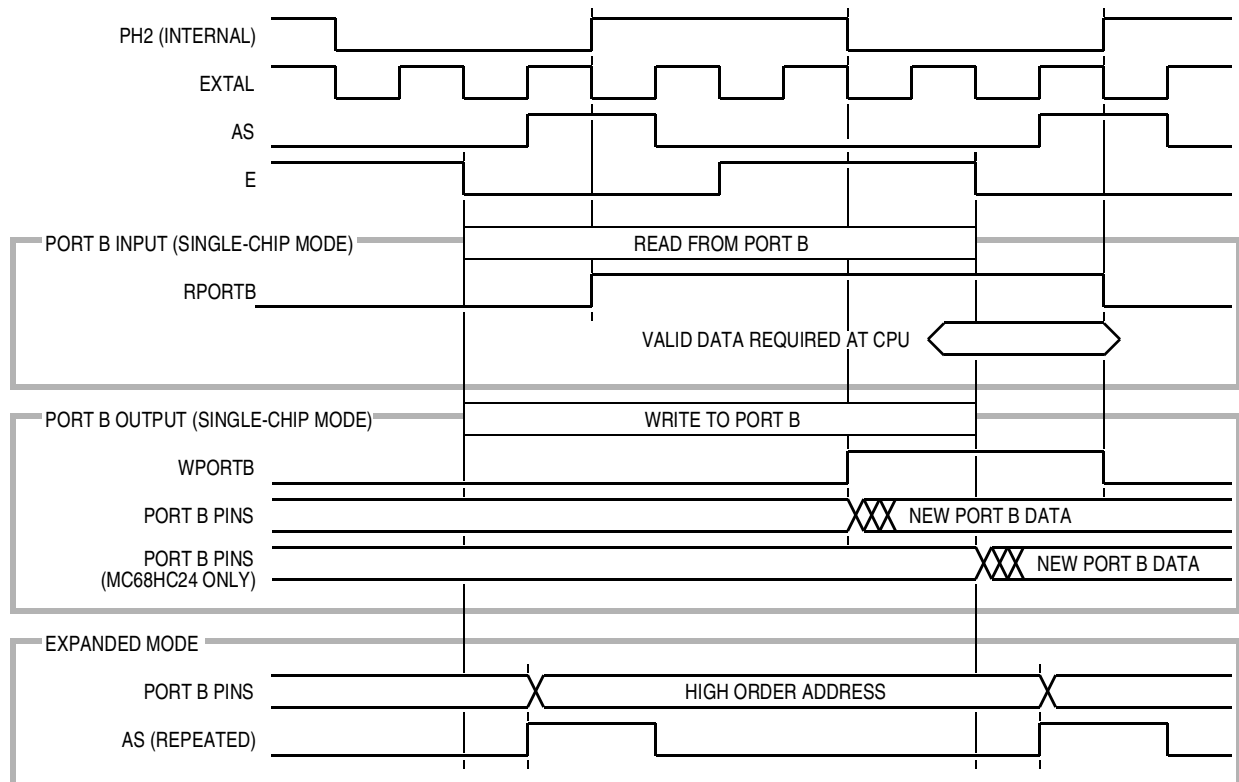
Figure 7-9. Idealized Port B Timing
