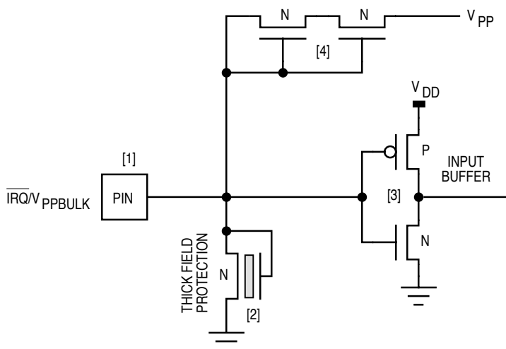
Figure 2-21. Internal Circuitry — \overline{\text{IRQ}}/\text{V}_{\text{PPBULK}} Pin
