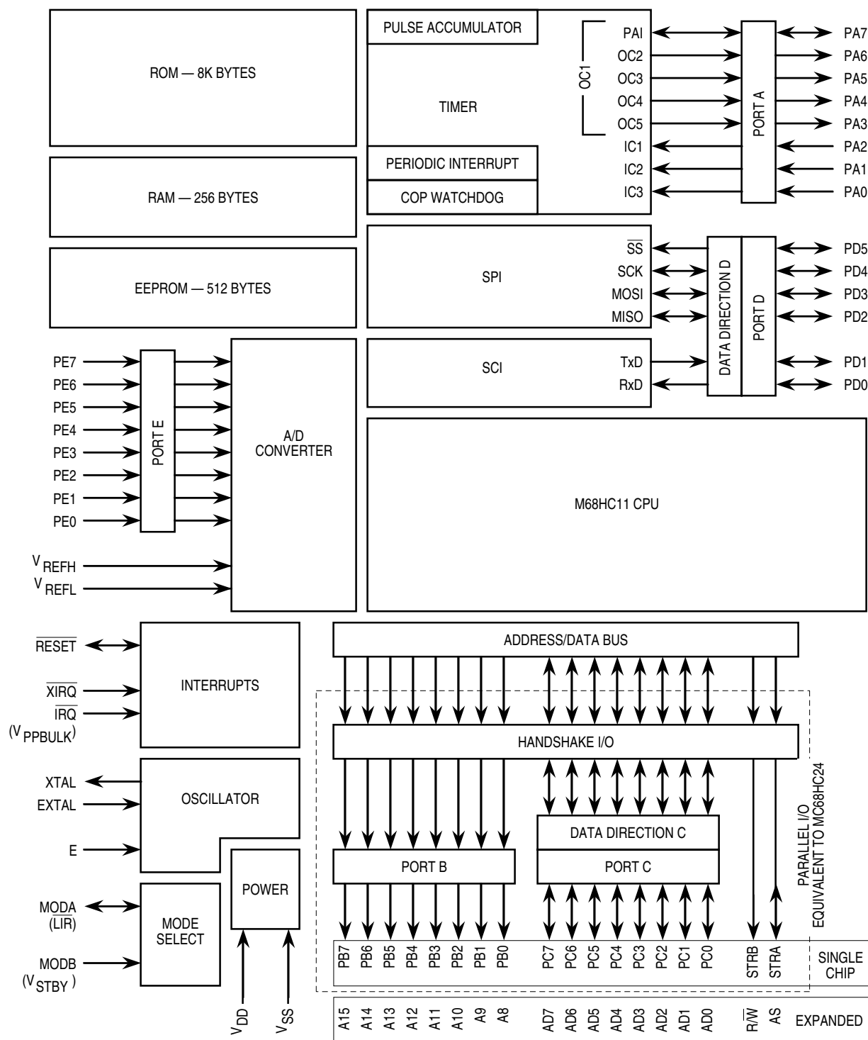
Figure 1-1. Block Diagram
