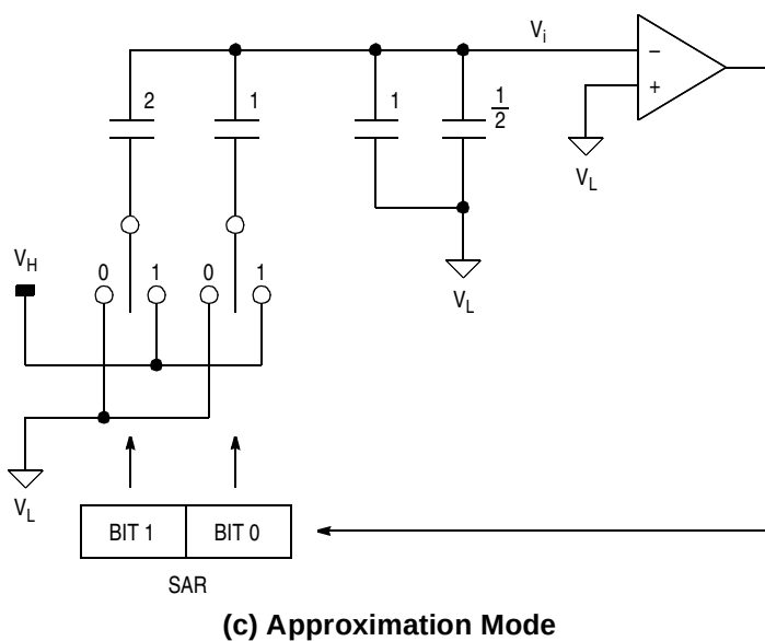
Figure 12-2. Charge-Redistribution A/D with \pm 1/2 LSB Quantization Error
