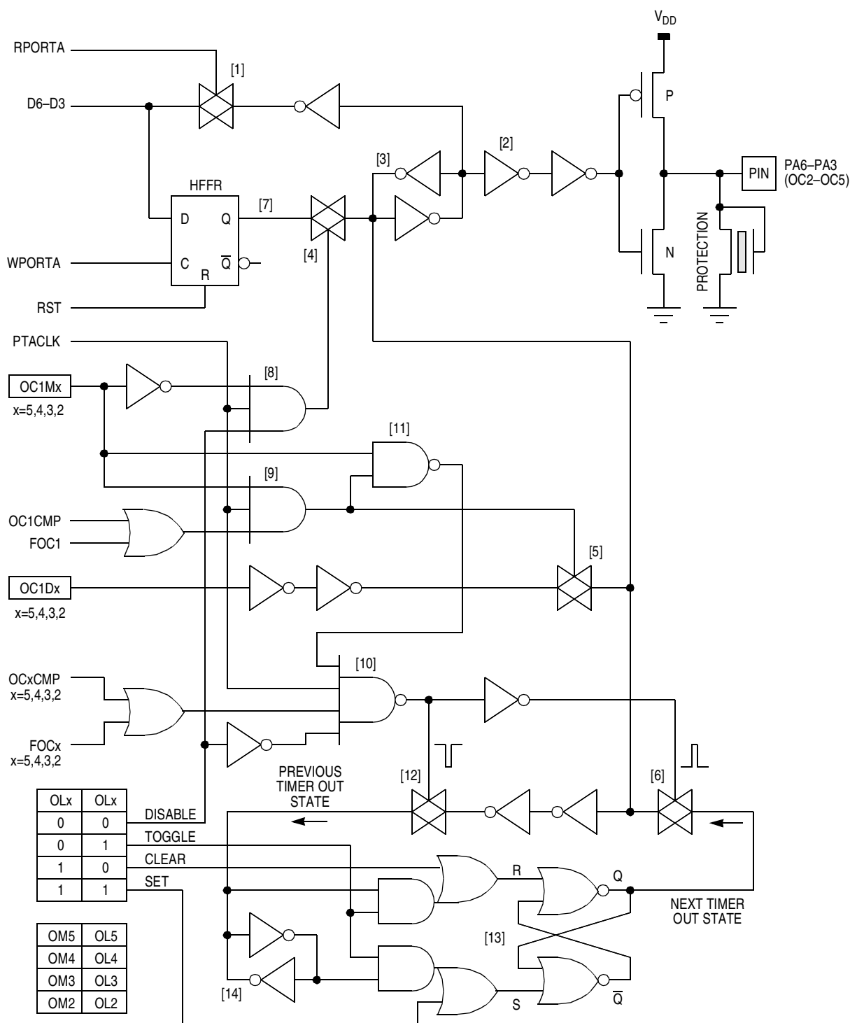
Figure 7-5. PA6-PA3 (OC5-OC2) Pin Logic
