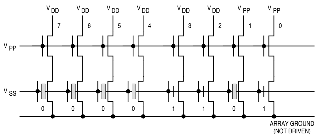
Figure 4-11. Selective-Write Programming Method
