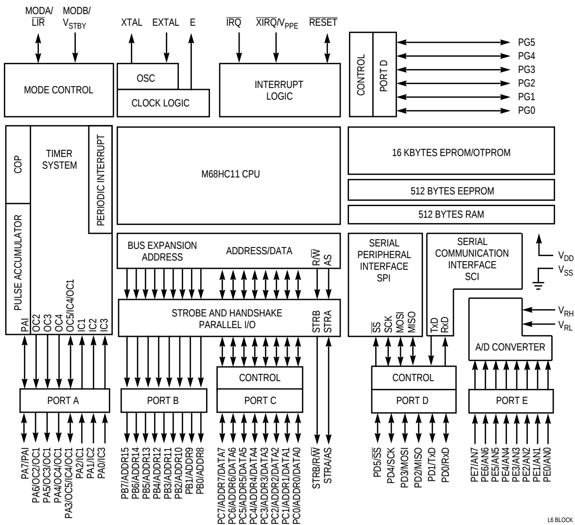
Figure 3 Block Diagram
