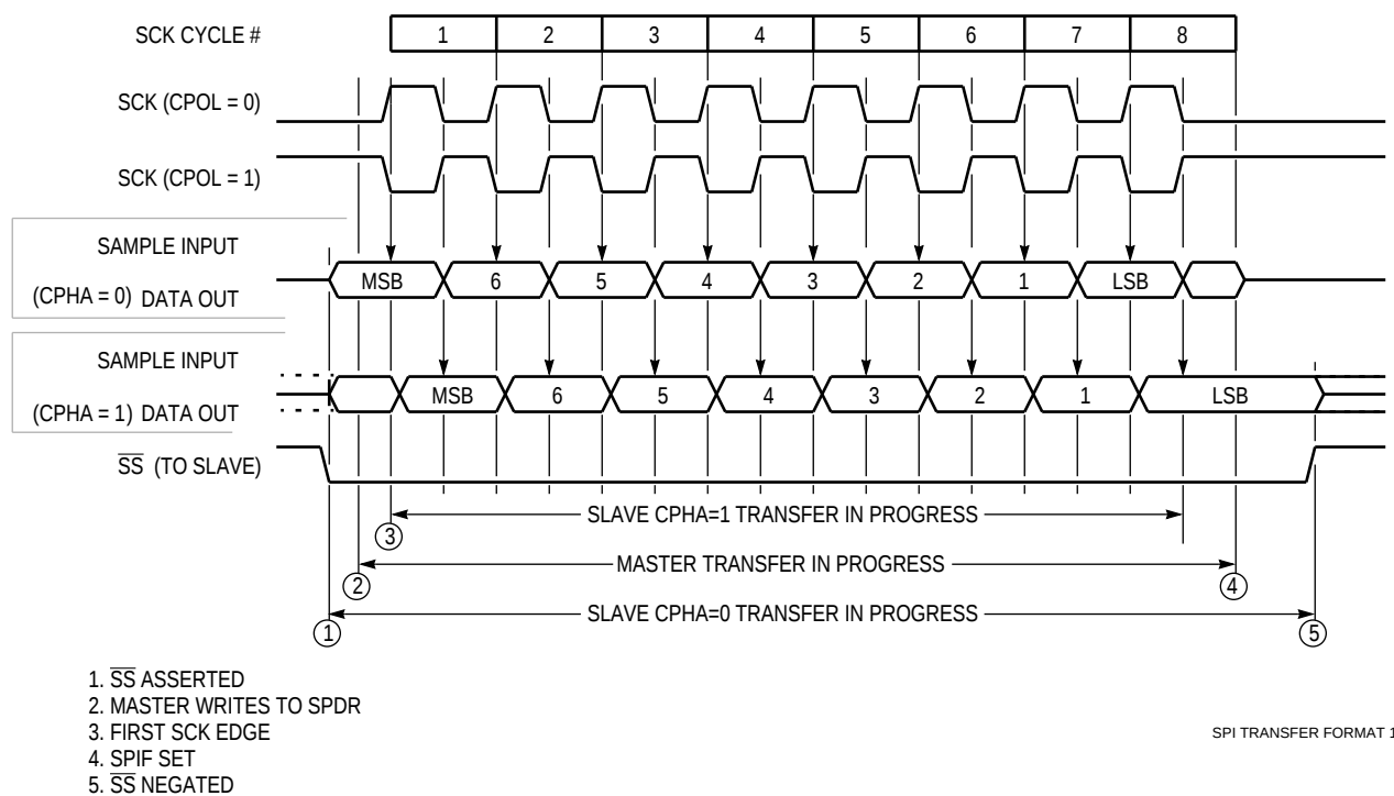
Figure 11 SPI Transfer Format
