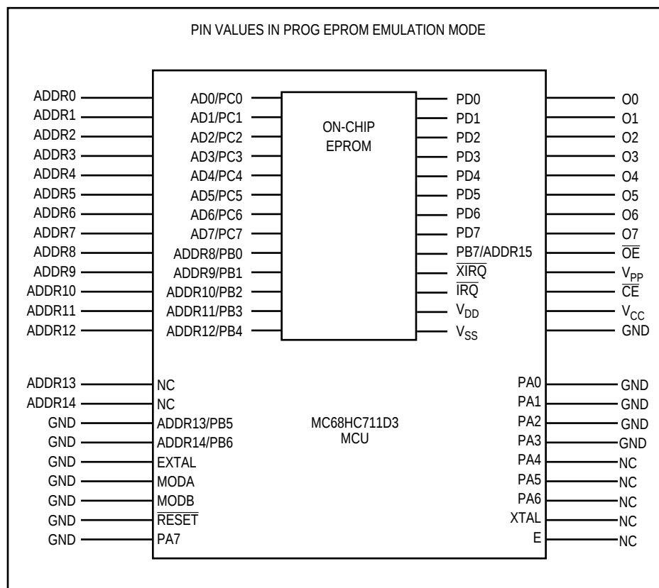
Figure 6 MC68HC711D3 Block Diagram — PROG Mode
