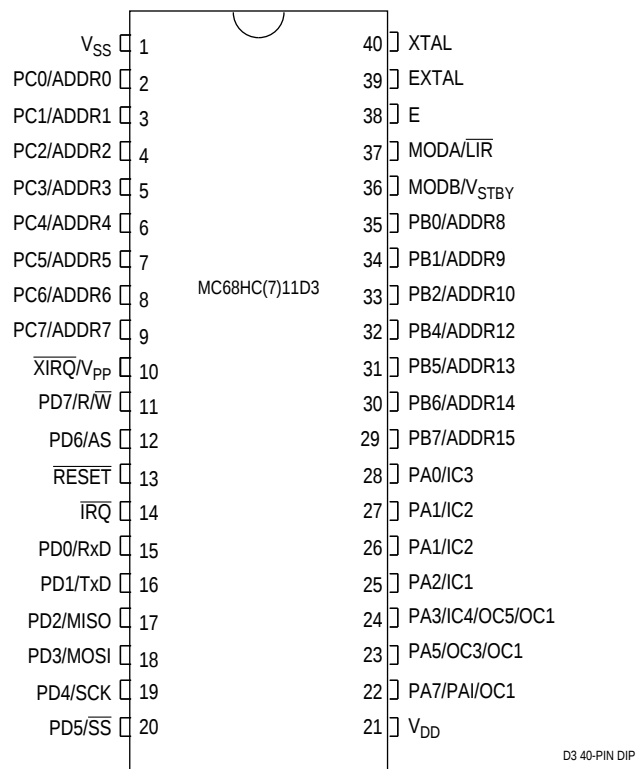
Figure 2 Pin Assignments for 40-Pin DIP
