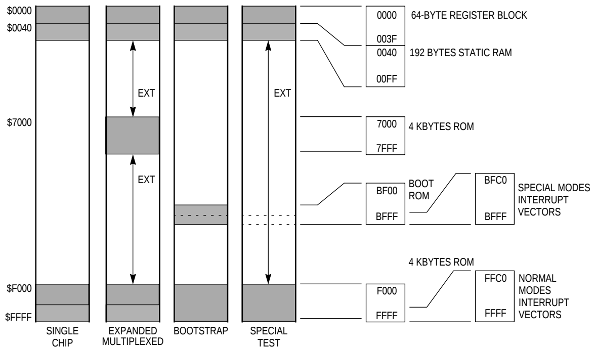
Figure 5 Memory Map
