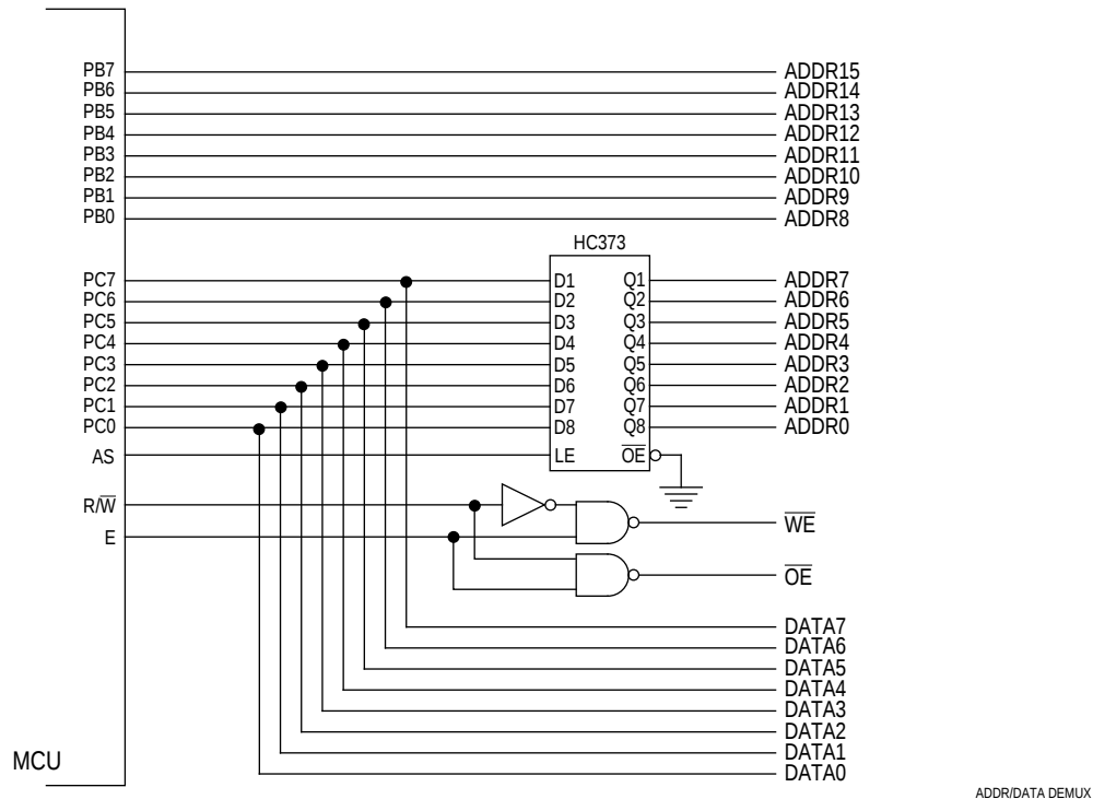
Figure 4 Address/Data Demultiplexing
