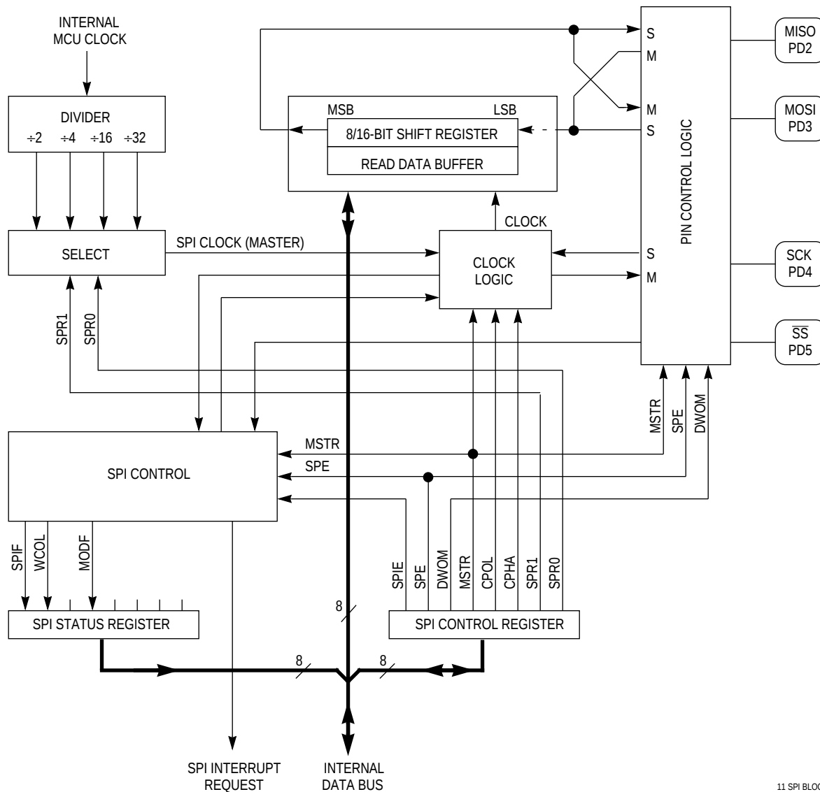
Figure 10 SPI Block Diagram
