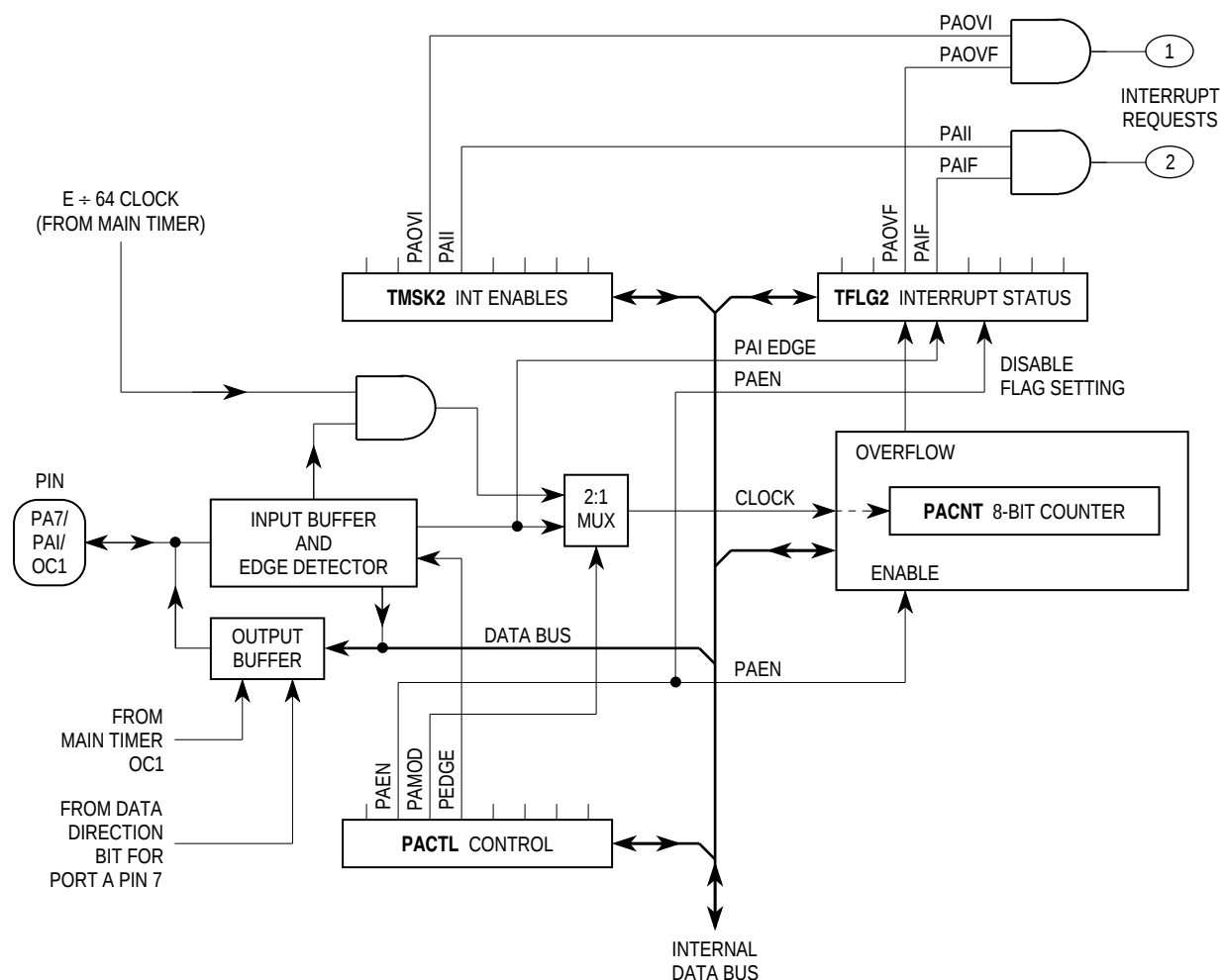
Figure 13 Pulse Accumulator System Block Diagram
