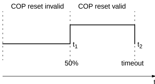
Figure 5-2 WCOP period
