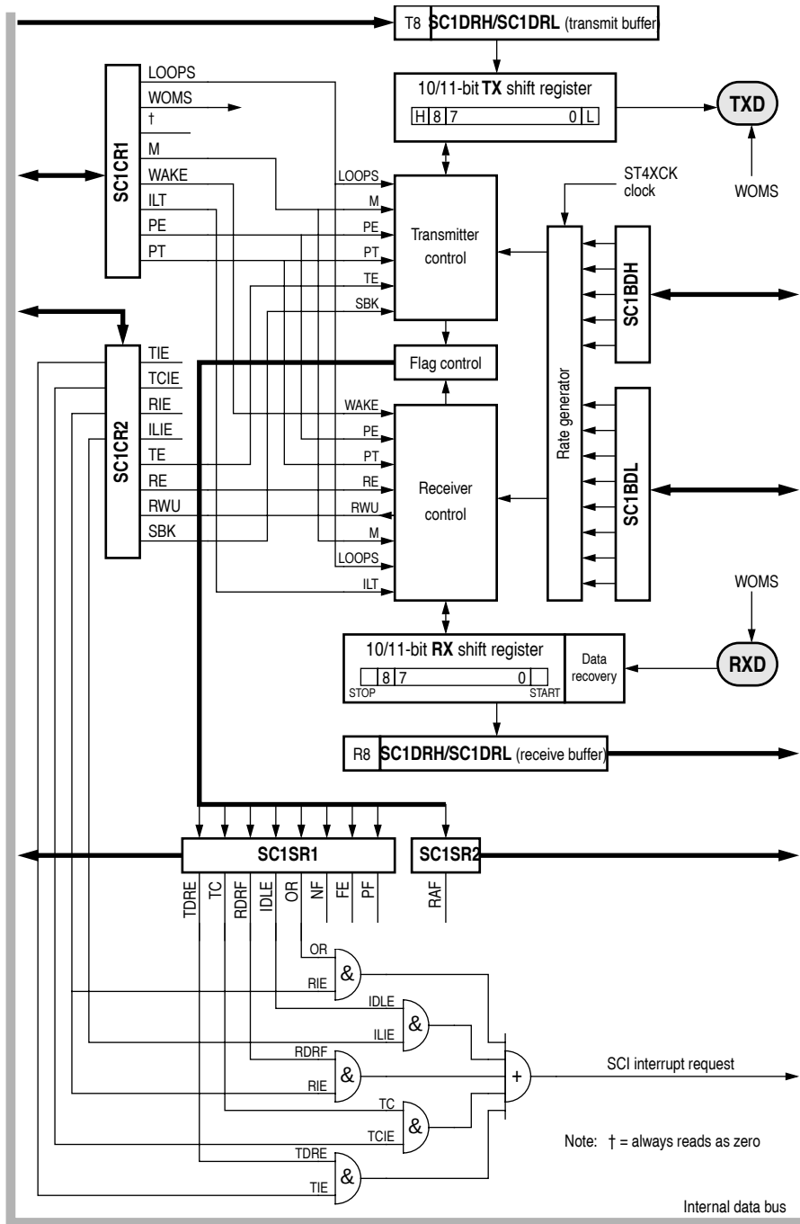
Figure 7-2 SCI1 block diagram
