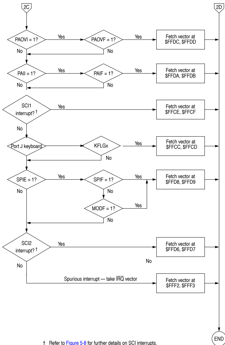
Figure 5-7 Interrupt priority resolution (3 of 3)
