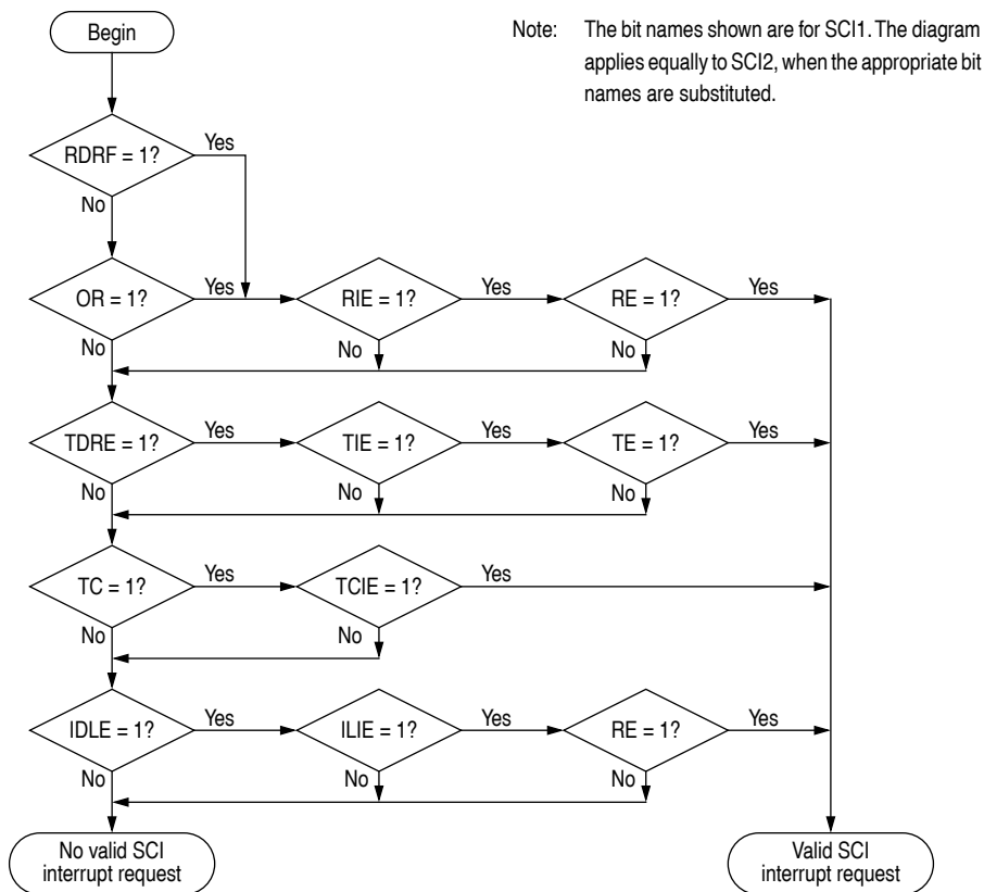
Figure 7-3 Interrupt source resolution within SCI1
