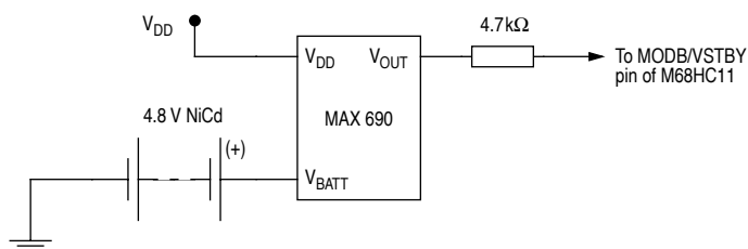
Figure 2-6 RAM stand-by connections
