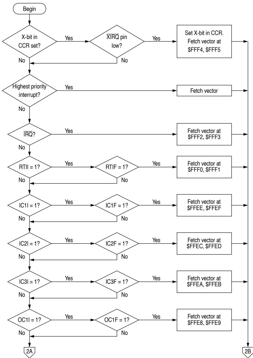
Figure 5-5 Interrupt priority resolution (1 of 3)
