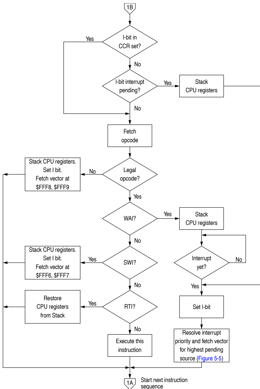
Figure 5-4 Processing flow out of reset (2 of 2)
