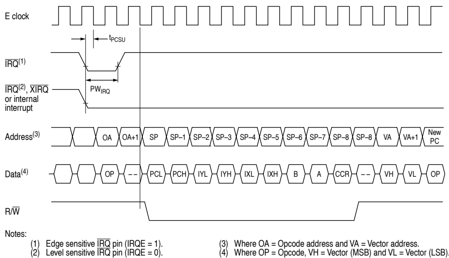
Figure A-4 Interrupt timing
