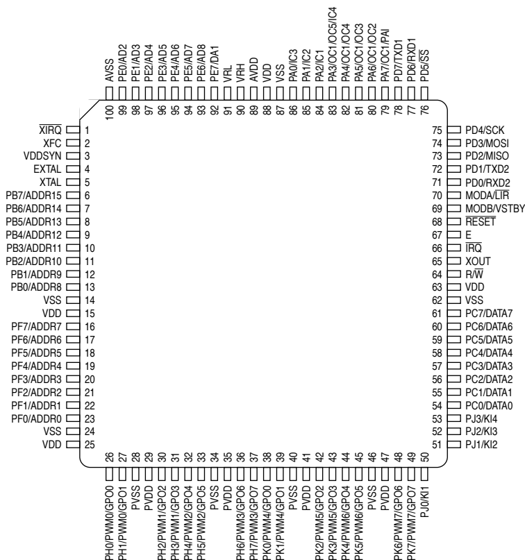
Figure 2-1 100-pin TQFP
