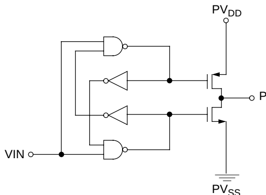
Figure 9-5 Power driver circuit
