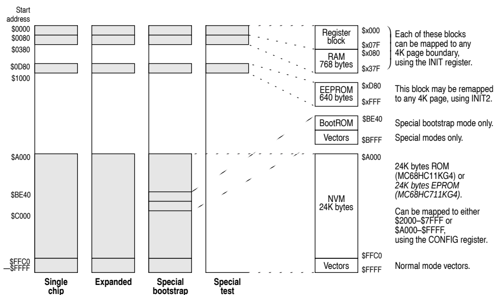
Figure 4-1 MC68HC11KG4 memory map
