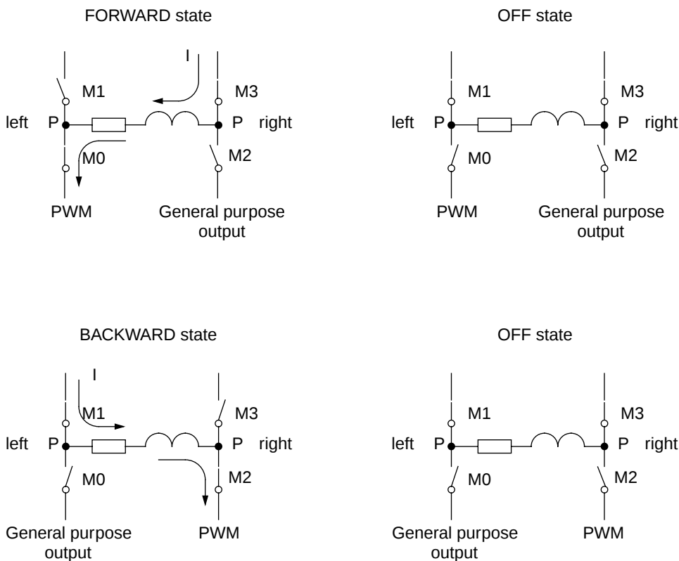
Figure 9-7 H-bridge states
