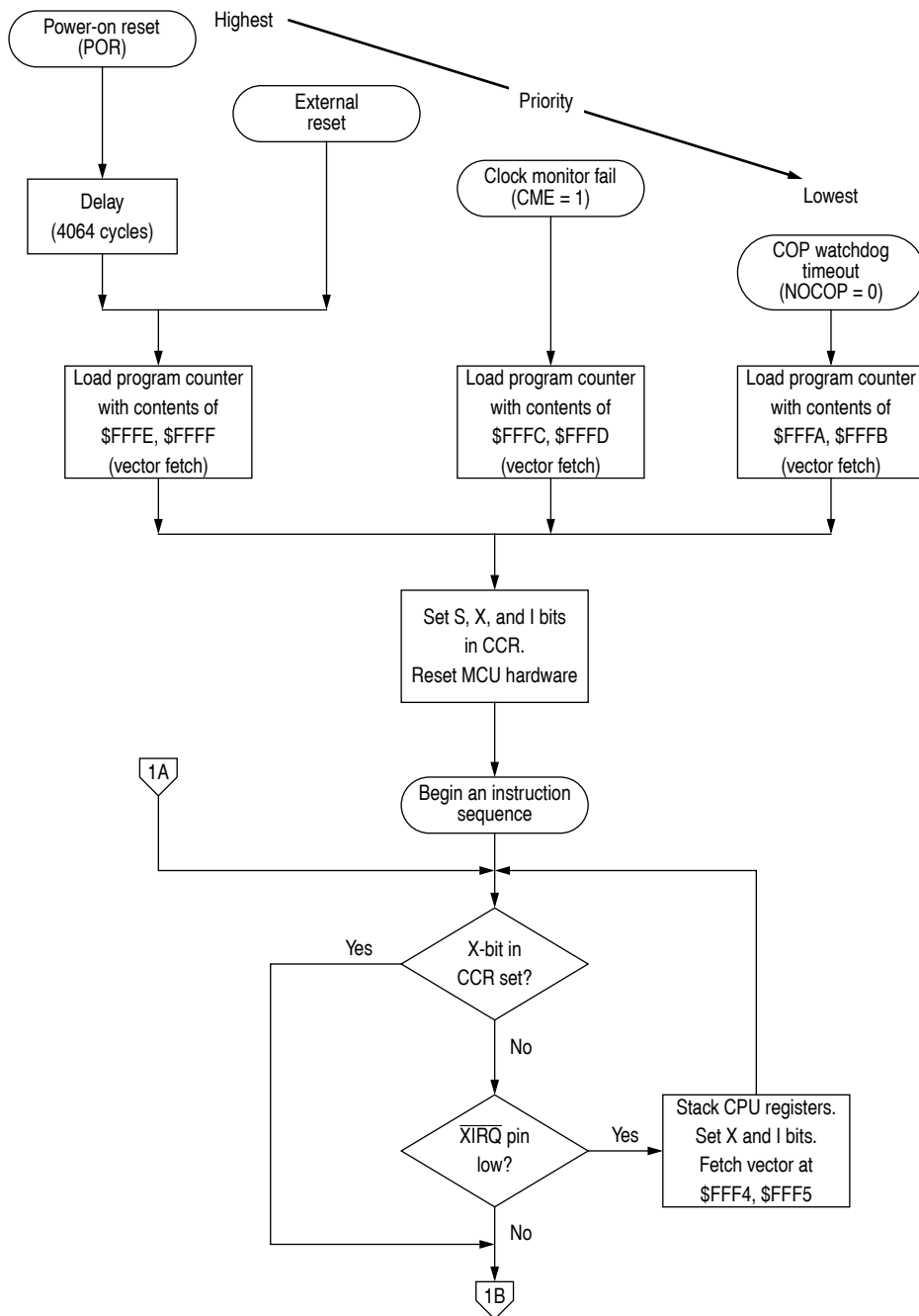
Figure 5-3 Processing flow out of reset (1 of 2)
