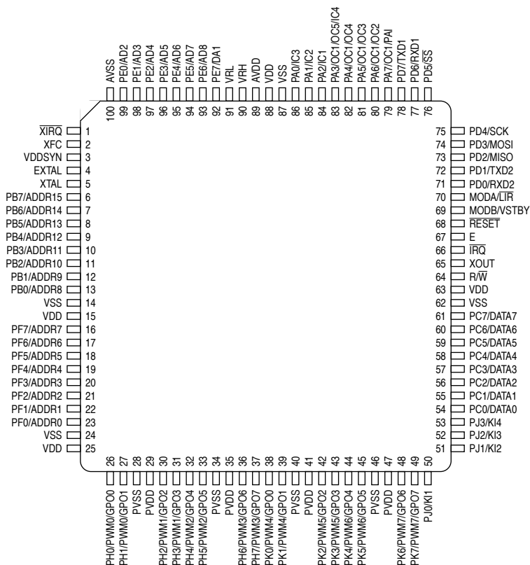
Figure B-1 100-pin TQFP
