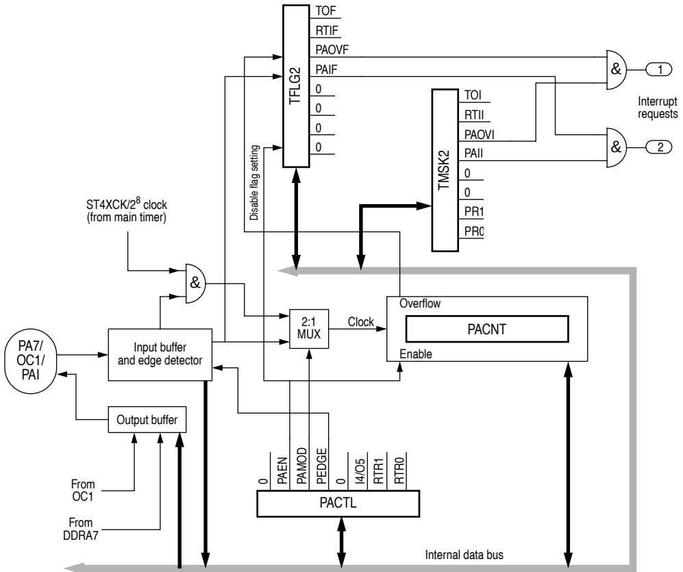
Figure 10-4 Pulse accumulator block diagram
