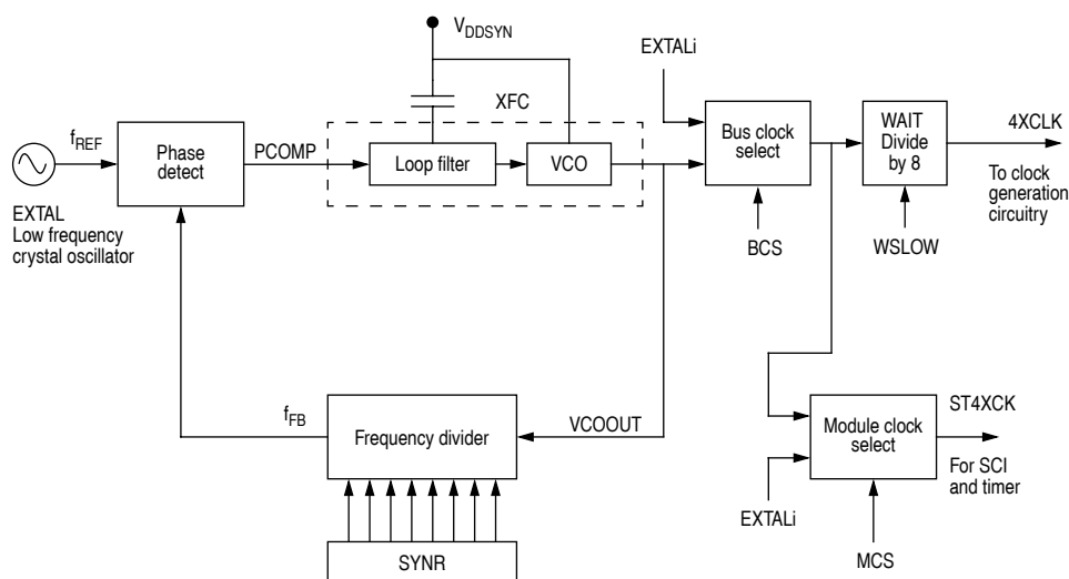
Figure 2-5 PLL circuit
