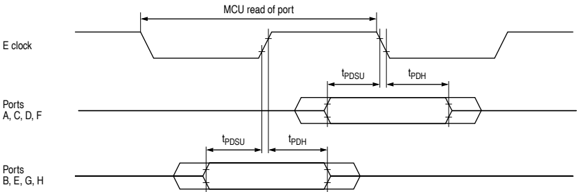
Figure 12-7 Port read timing diagram
