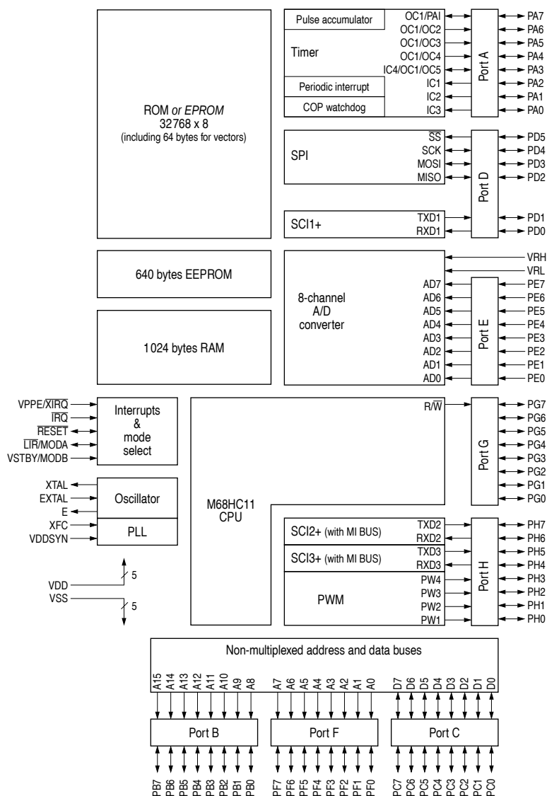
Figure 1-1 MC68HC11P2/MC68HC711P2 block diagram
