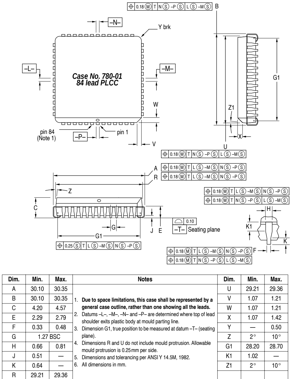
Figure 13-3 84-pin PLCC mechanical dimensions
