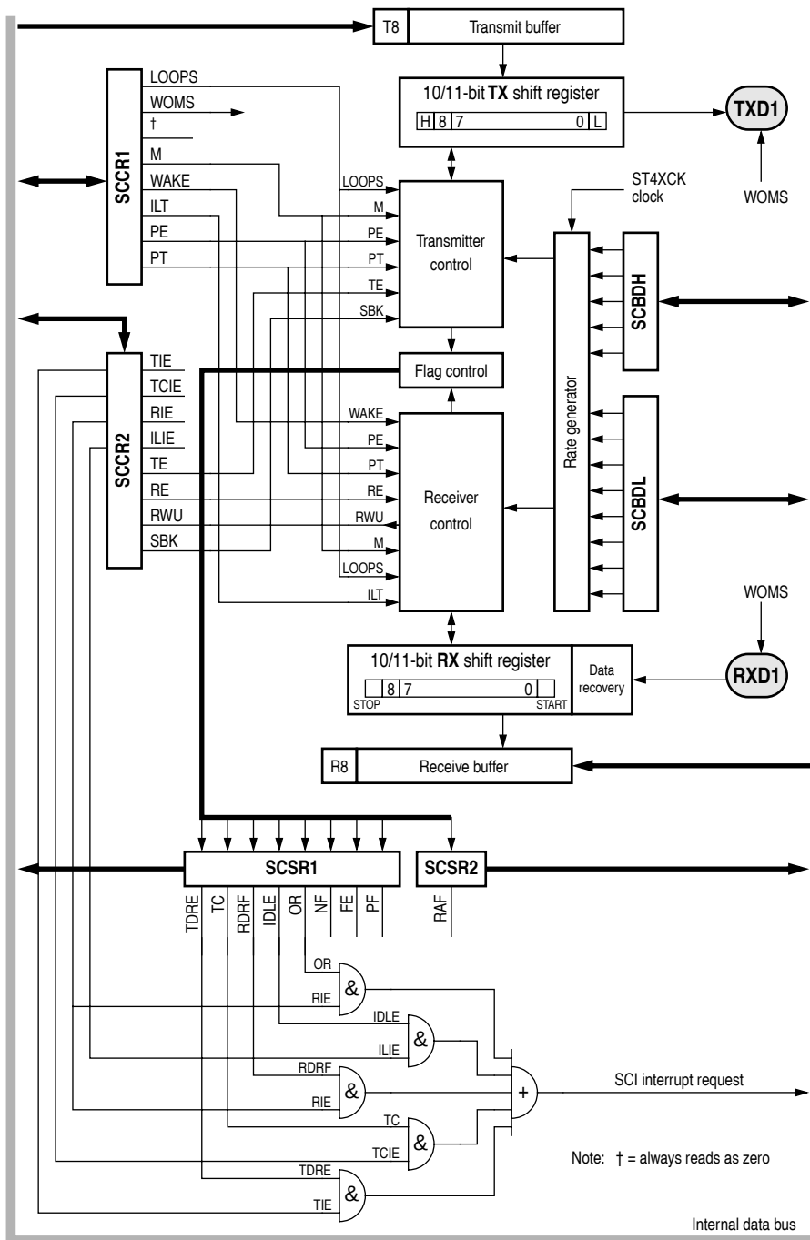
Figure 5-2 SCI1 block diagram
