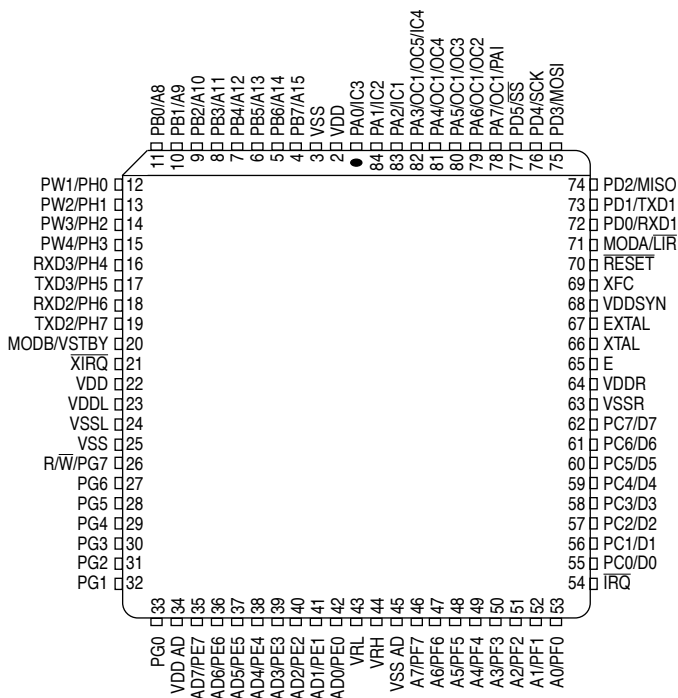
Figure 13-1 84-pin PLCC/CERQUAD pinout
