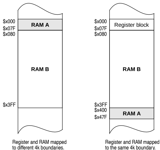
Figure 3-2 RAM and register overlap
