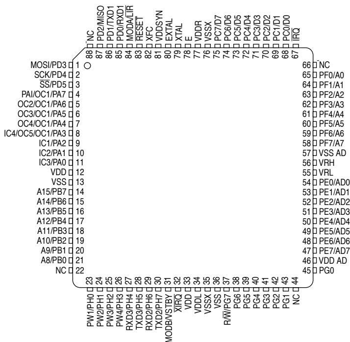
Figure 2-2 88-pin QFP pinout
