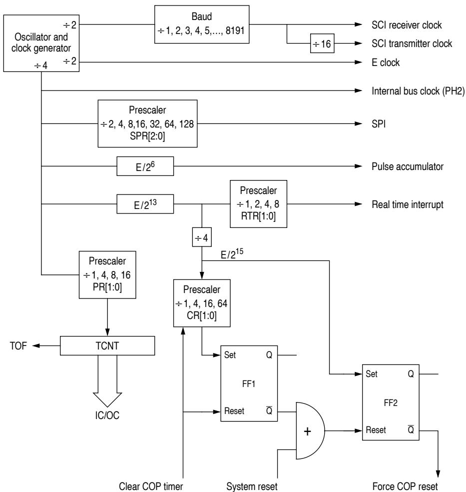
Figure 8-1 Timer clock divider chains
