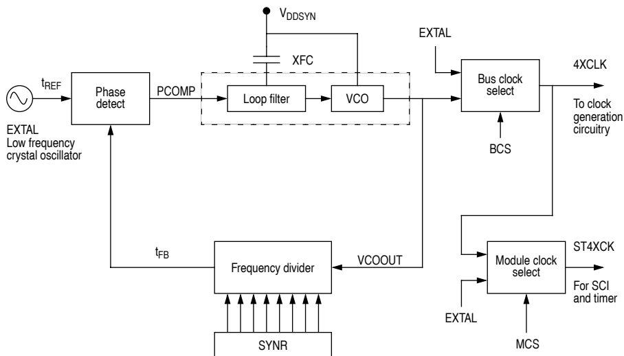
Figure 2-5 PLL circuit
