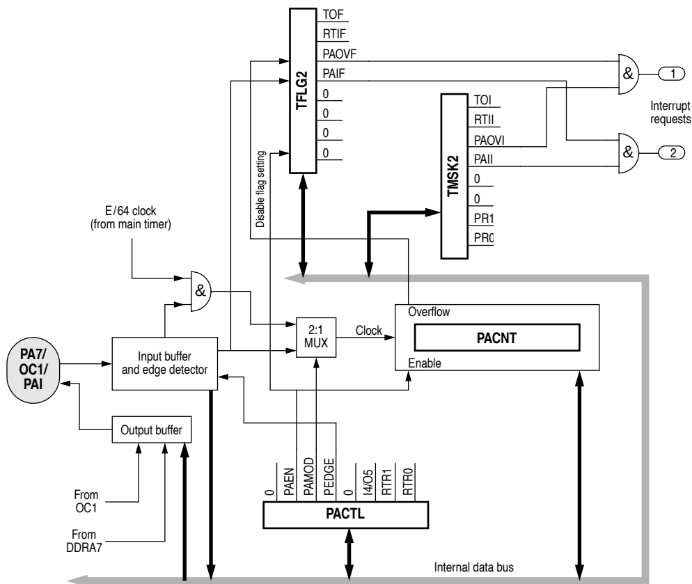
Figure 8-3 Pulse accumulator block diagram
