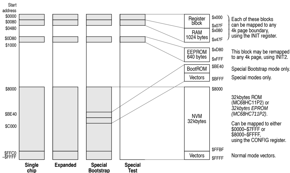
Figure 3-1 MC68HC11P2 memory map
