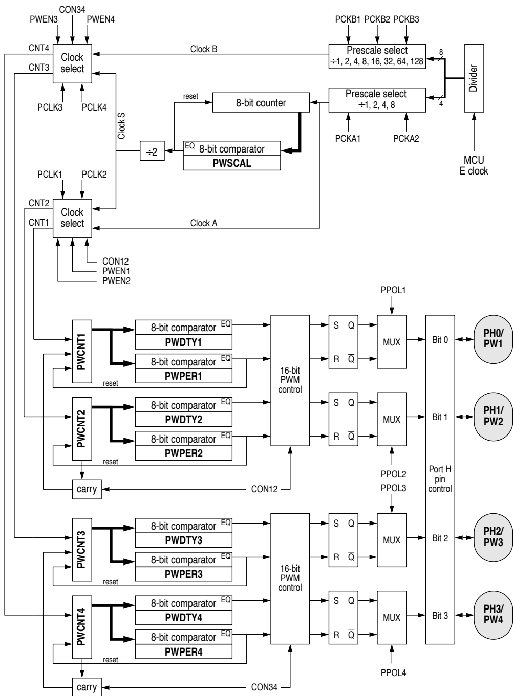
Figure 8-4 PWM timer block diagram
