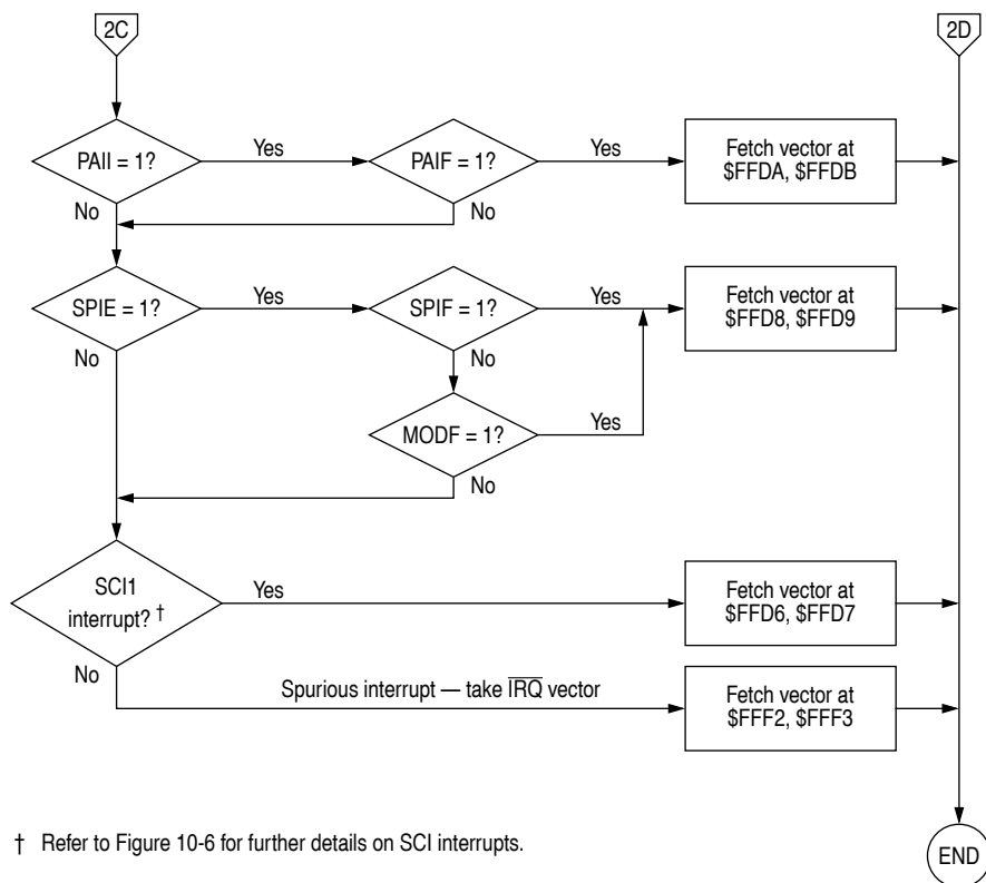
Figure 10-5 Interrupt priority resolution (3 of 3)
