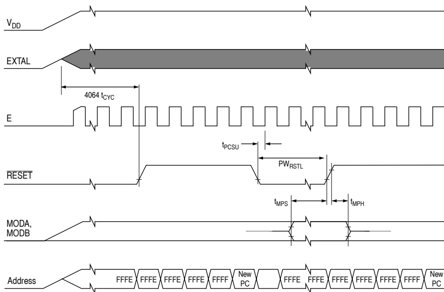
Figure 12-3 Reset timing
