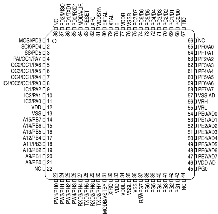
Figure 13-2 88-pin QFP pinout
