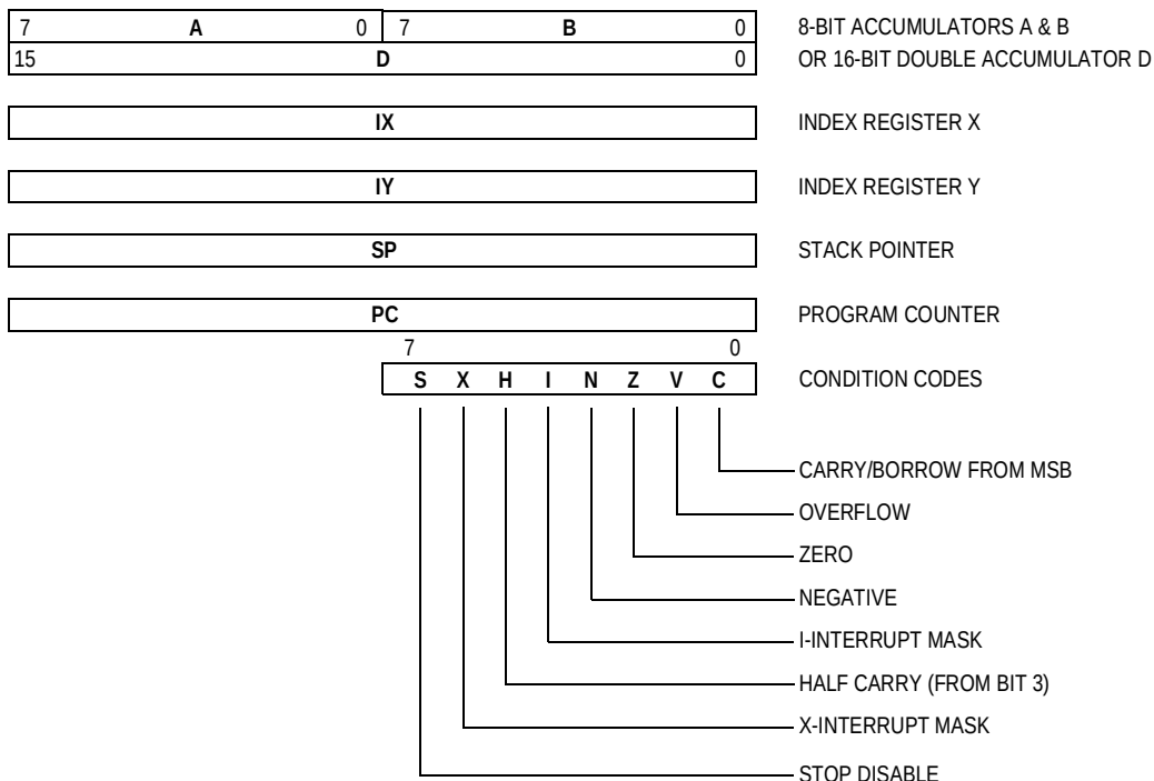
Figure 3-1. Programming Model
