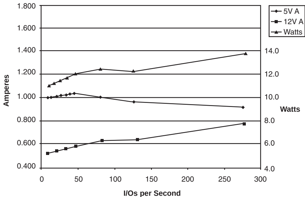
Figure 10. ST318452 DC current and power vs. input/output operations per second (LVD)
