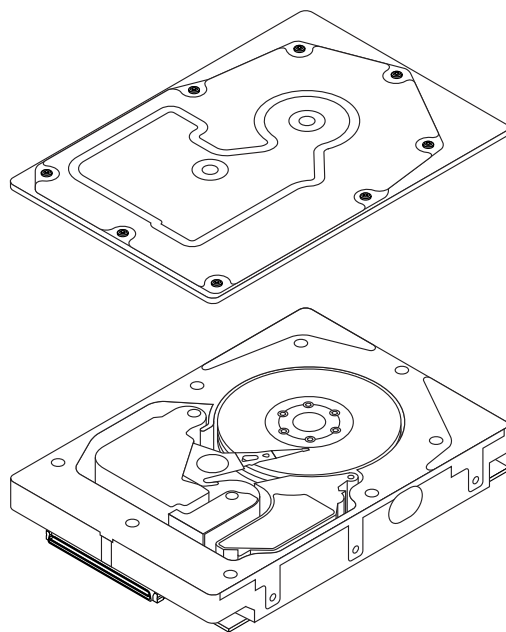
Figure 2. Cheetah X15 36LP family drive (exploded view)
