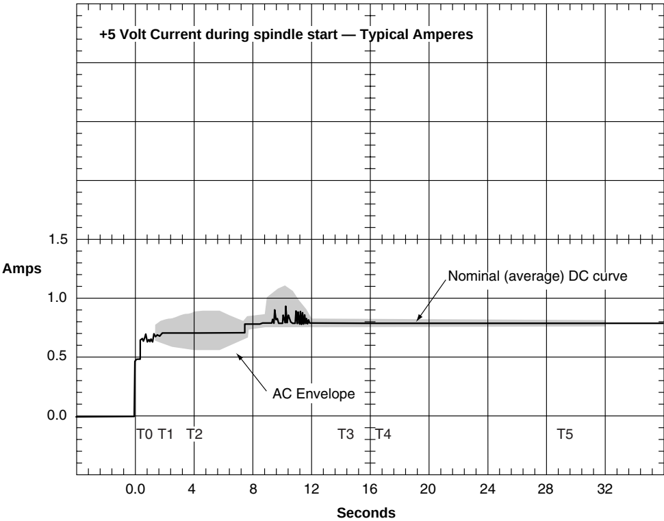
Figure 4. Typical ST336752 drive +5 V current profile
