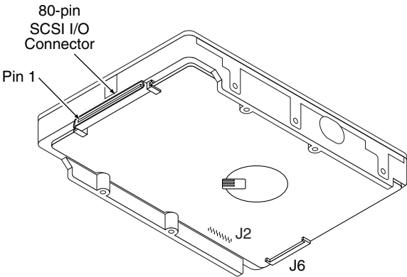
Figure 20. LC model drive physical interface (80-pin J1 SCSI I/O connector)
