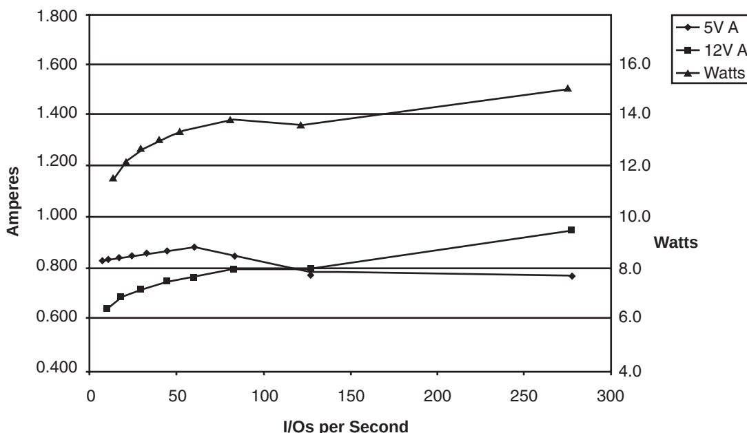
Figure 7. ST336752 DC current and power vs. input/output operations per second (SE)
