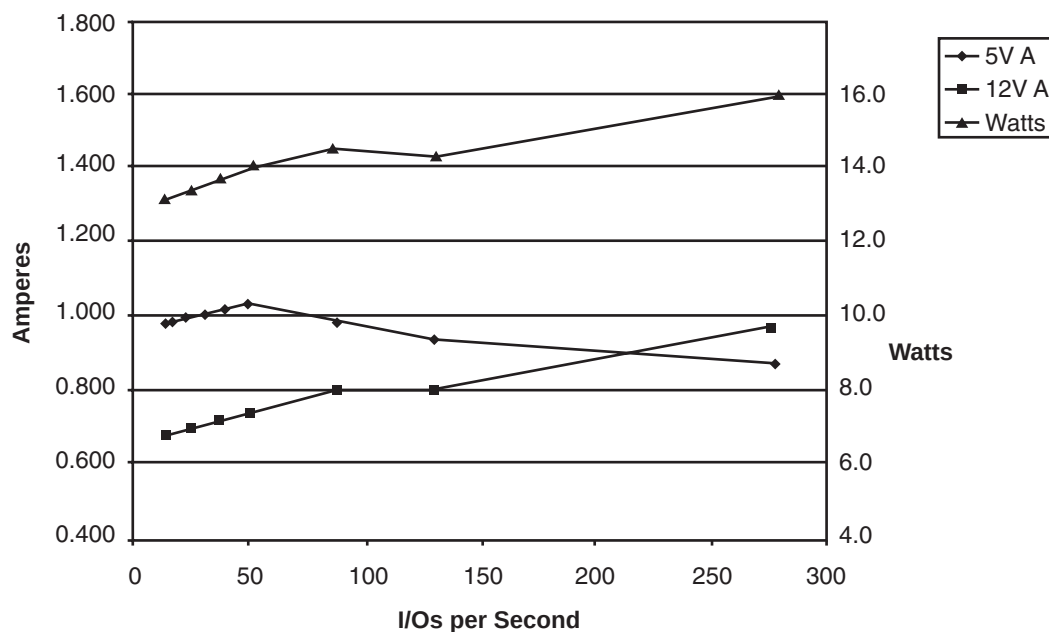
Figure 8. ST336752 DC current and power vs. input/output operations per second (LVD)
