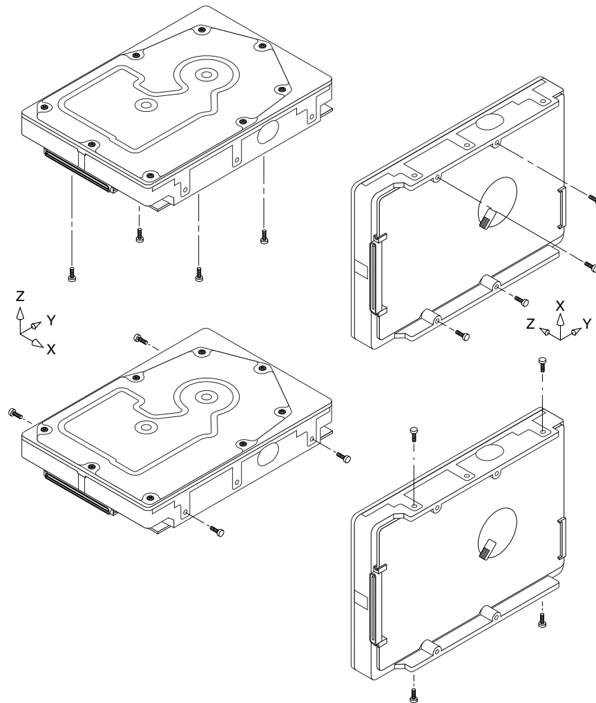
Figure 12. Recommended mounting
