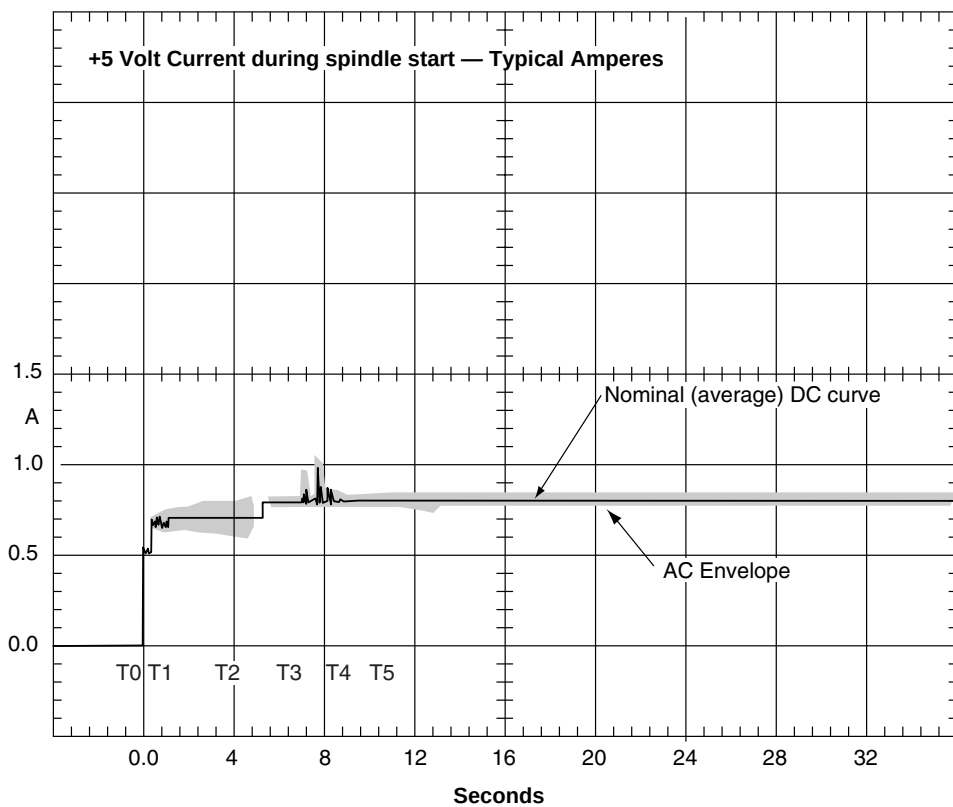
Figure 6. Typical ST318452 drive +5 V current profile
