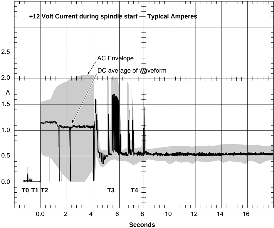
Figure 5. Typical ST318452 drive +12 V current profile
