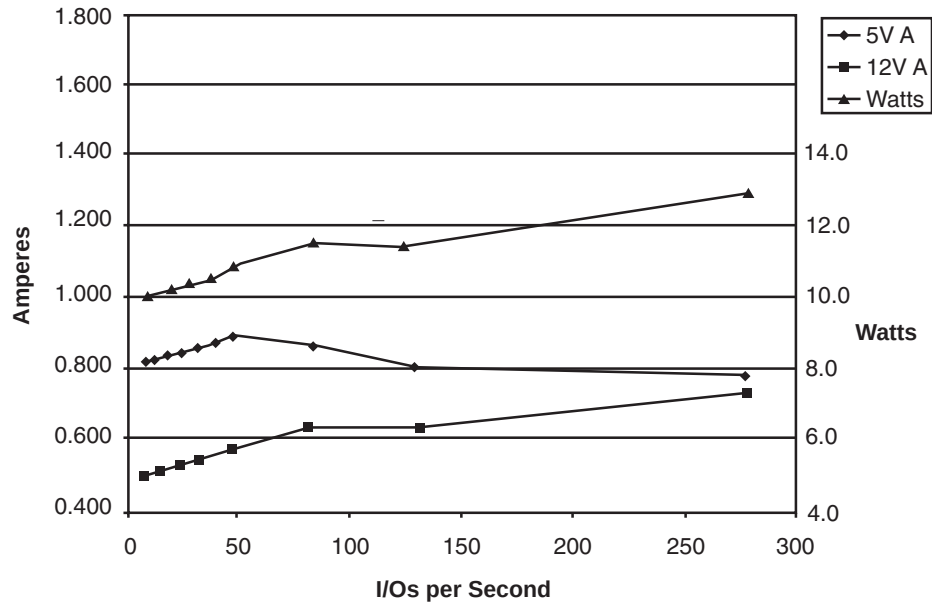
Figure 9. ST318452 DC current and power vs. input/output operations per second (SE)
