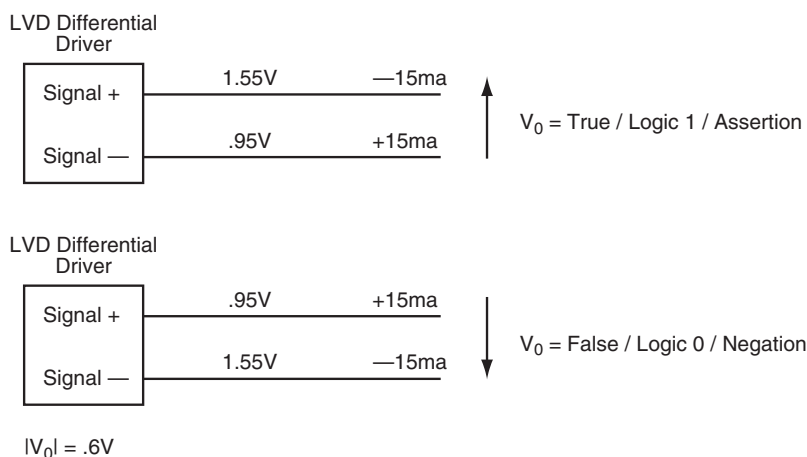
Figure 24. LVD output signals
