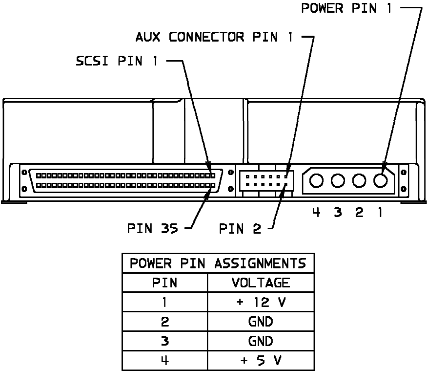
Figure 27. Electrical connectors (rear view) -- 68 pin models.
