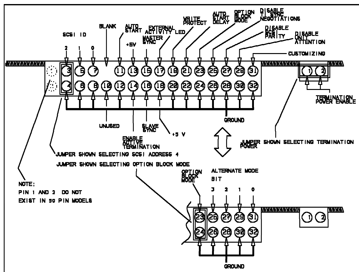
Figure 30. 50 pin Single Ended Front Option Jumper Block (& TermPower Block)
