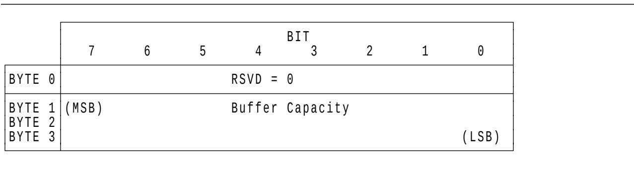
Figure 67. READ BUFFER Header
