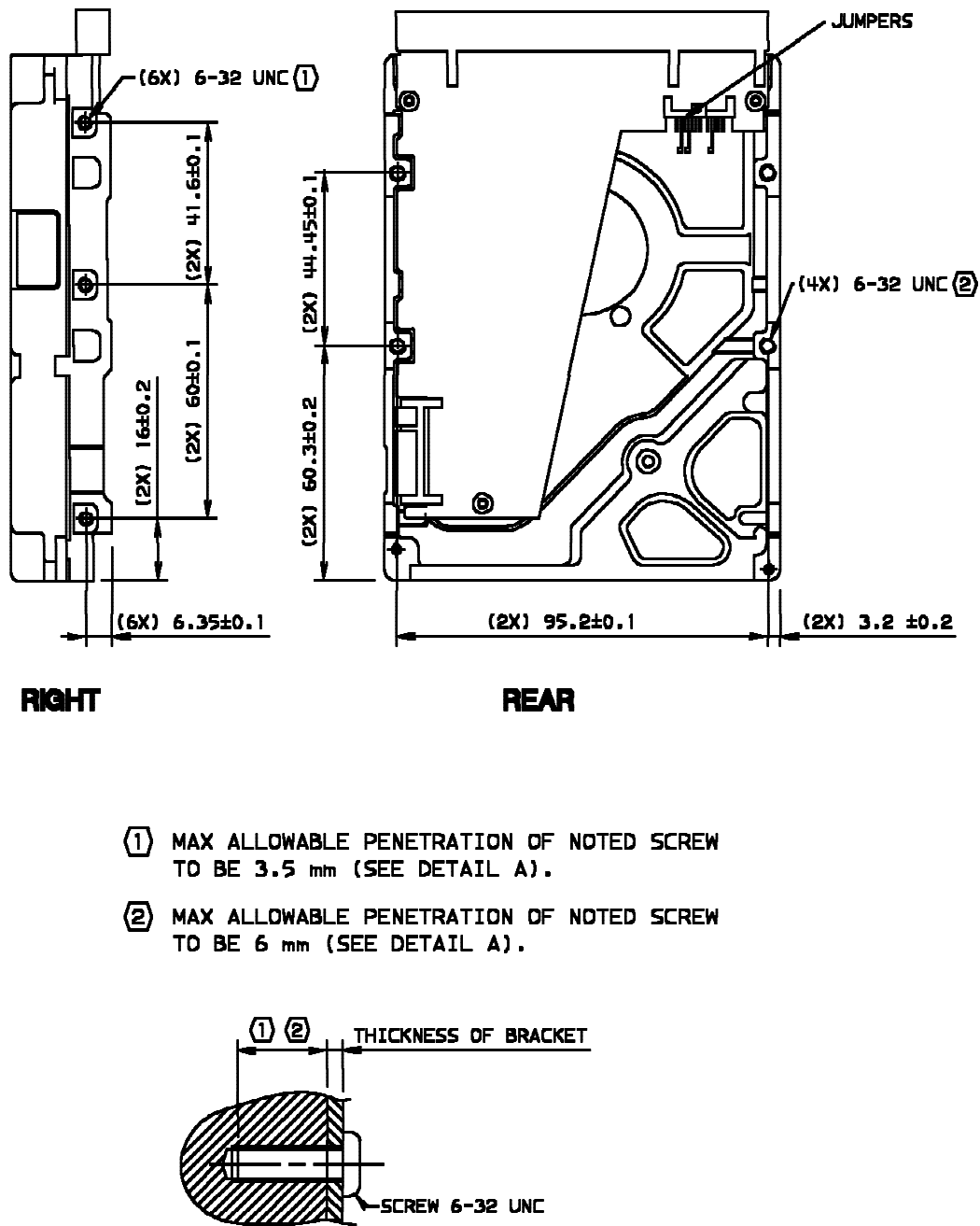
Figure 17. Mounting Positions and the Tappings
