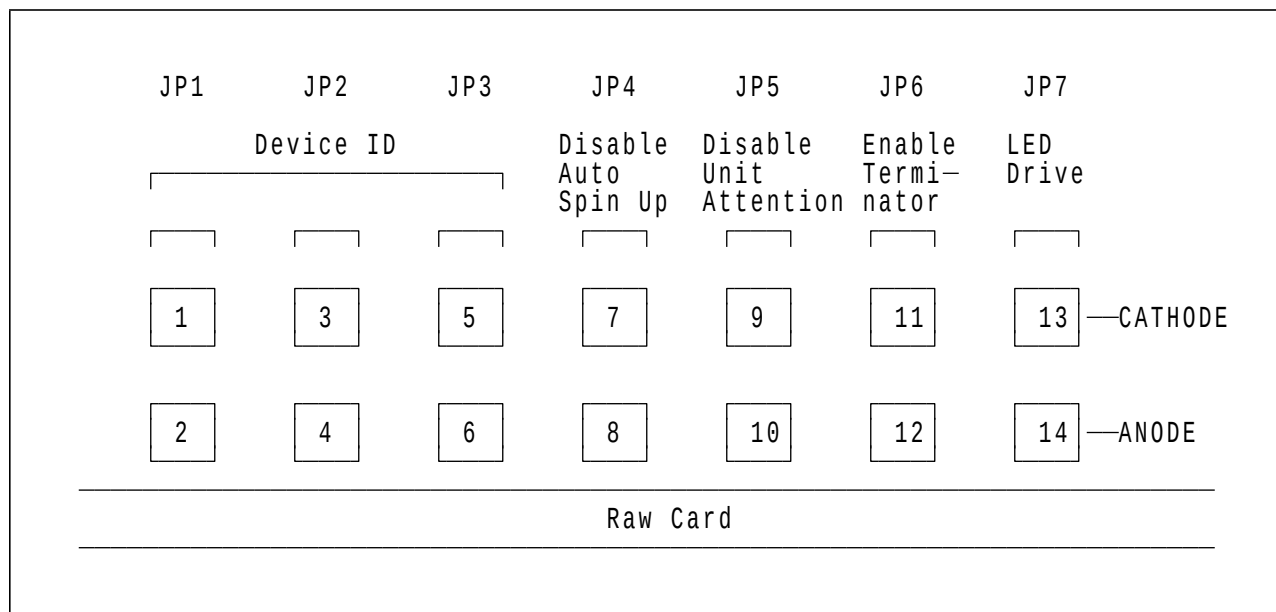
Figure 26. Jumper Pins
