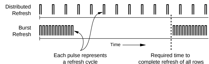
Figure 1 BURST AND DISTRIBUTED REFRESH
