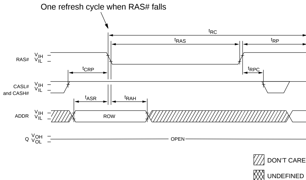
Figure 2 RAS#-ONLY REFRESH
