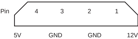
Figure 3-2 Power Connector
