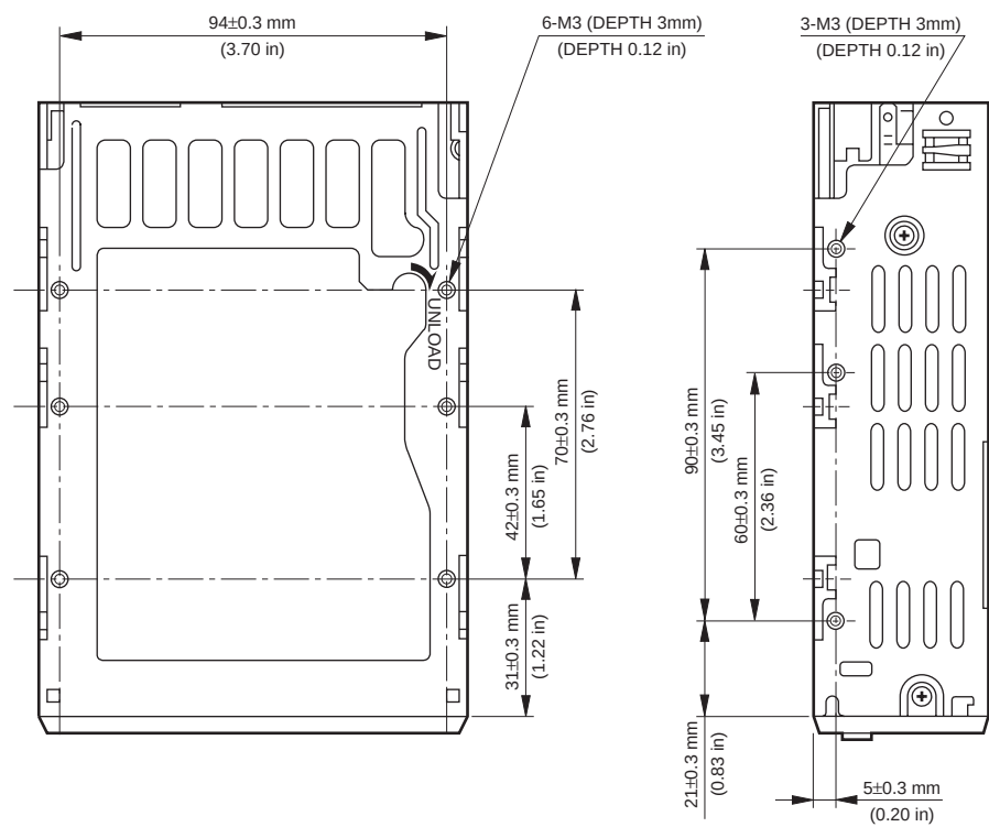
SDT-9000 Figure 2-2 Mounting Holes
