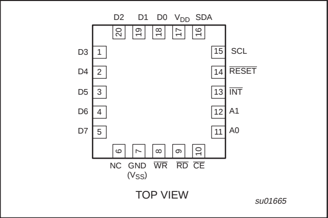
PIN CONFIGURATION — HVQFN
