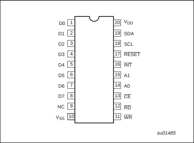
PIN CONFIGURATION
